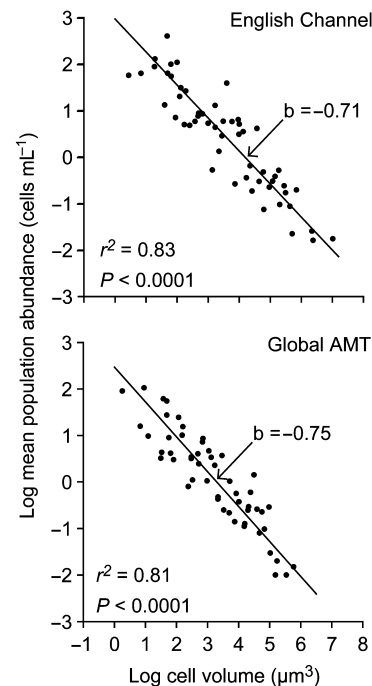
Figure 1 Relationship between log mean population abundance and log cell volume of phytoplankton species from the English Channel and the Atlantic Meridional Transects. Each data point represents the most abundant species in each size class of width 0.1 log cell volume.
