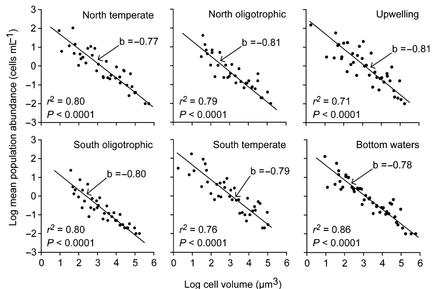
Figure 2 Relationship between log mean population abundance and log cell volume of phytoplankton species from different ocean regions along the Atlantic Meridional Transects. Each data point represents the most abundant species in each size class of width 0.1 log cell volume.
